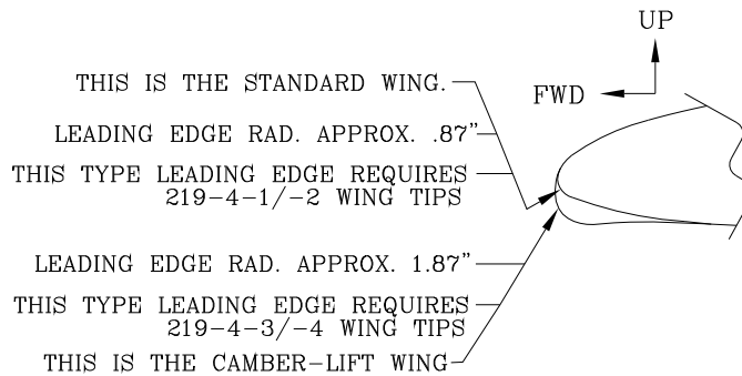
FIGURE 1 SHOWING LEADING EDGE OF WING
